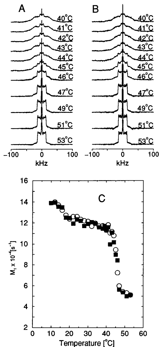
FIGURE 7 (A) ^2\text{H} NMR spectra at selected temperatures for DPPC/DPPG- d_{62} (7:3) in the presence of 5 mM \text{Ca}^{2+} . (B) ^2\text{H} NMR spectra at selected temperatures for DPPC/DPPG- d_{62} (7:3) with 10% (w/w) SP-C in the presence of 5 mM \text{Ca}^{2+} . (C) Temperature dependence of ^2\text{H} -NMR first spectral moments for (○) DPPC/DPPG- d_{62} (7:3) in the presence of 5 mM \text{Ca}^{2+} and (■) DPPC/DPPG- d_{62} (7:3) with 10% (w/w) SP-C in the presence of 5 mM \text{Ca}^{2+} . Buffer is 135 mM NaCl, 15 mM HEPES.
